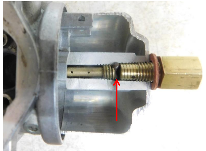
DAMAGED O-RING
